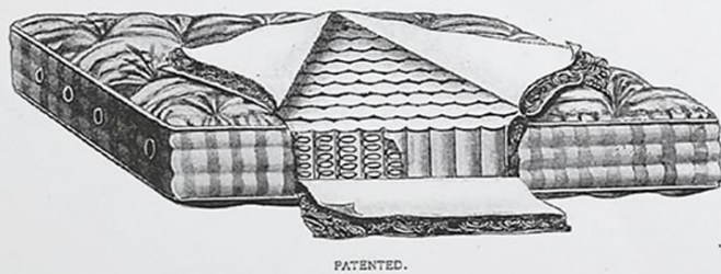
Opened Section showing Naked Springs; series of Pockets enclosing Springs; Casing turned back; Curled Hair Upholstering; Outside Tick, and Ventilators at End of Mattress.
